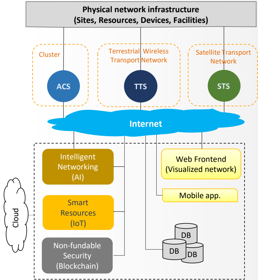
Network management process in O2I system
