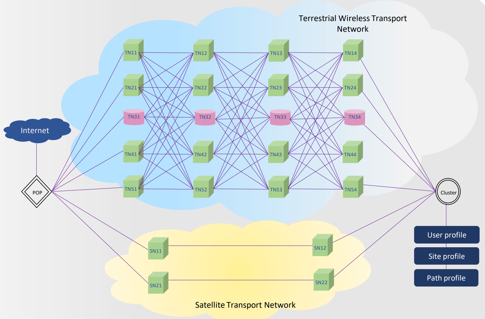
Logical network configuration on network abstraction
